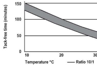
Figure 3: DOWSIL 993 Structural Glazing Sealant - Tack-free time range
