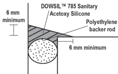
Figure 1: Fillet Joint
