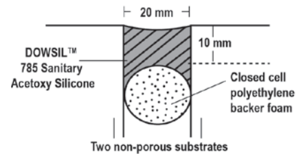
Figure 2: Deep Joint
