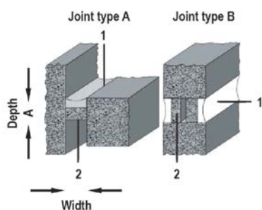
Figure 1: Test joint configurations
